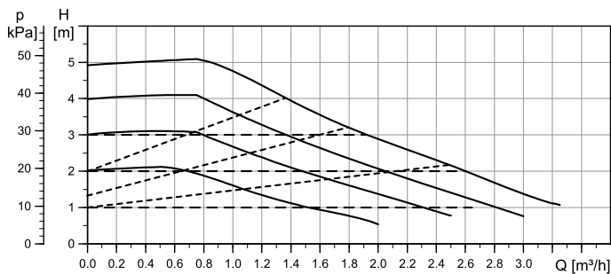
CAPACITY DIAGRAM
