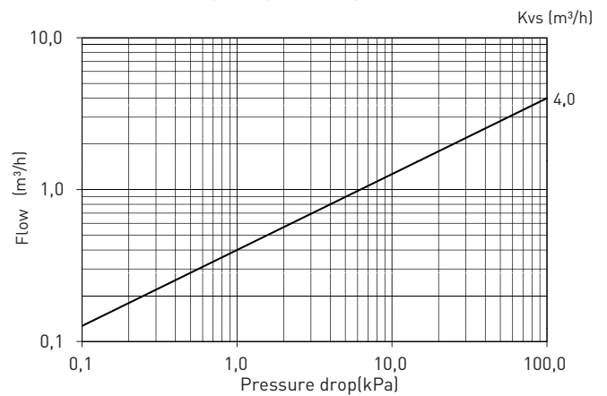
CAPACITY DIAGRAM
