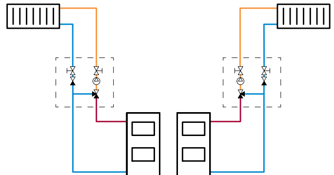
PUMP GROUP WITH MIXING VALVE
