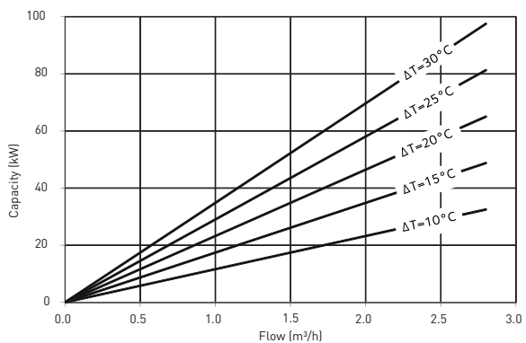
BOILER CAPACITY DIAGRAM, YONOS PARA*/6 RKC
