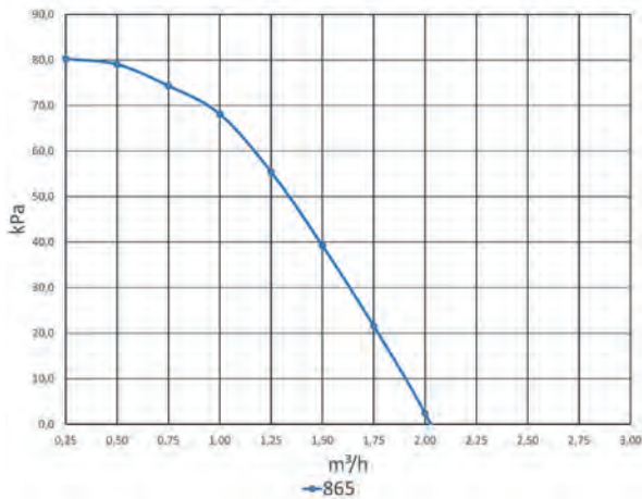
LK 865 - PUMP CHARACTERISTICS
