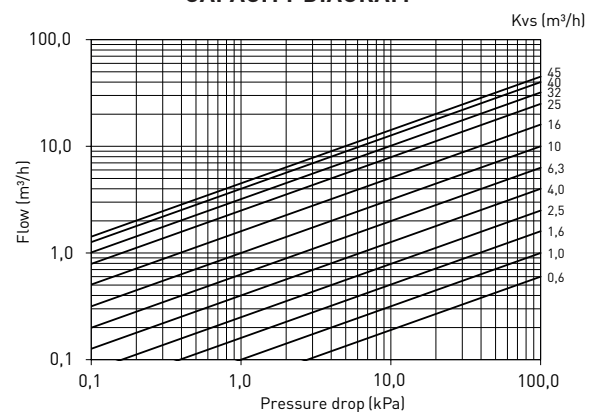
CAPACITY DIAGRAM
