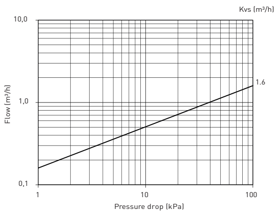
CAPACITY DIAGRAM
