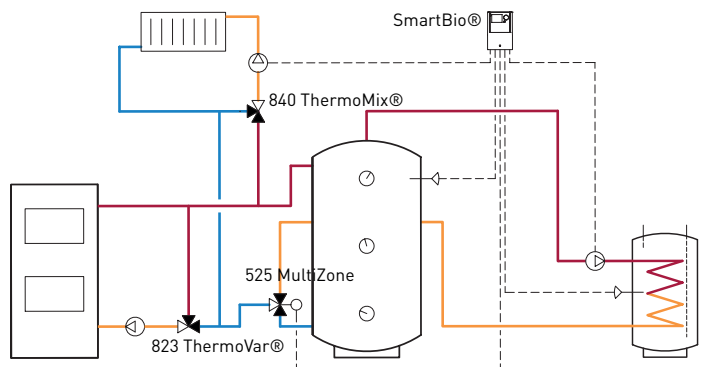
HYDRAULIC SYSTEM 4
