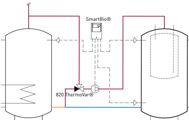
HYDRAULIC SYSTEM 2
