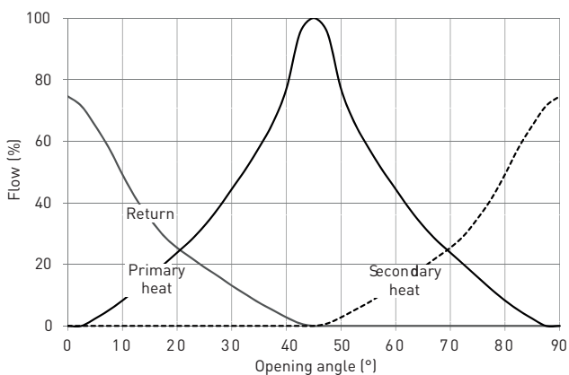
VALVE CHARACTERISTICS
