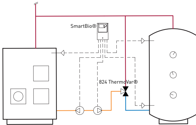
HYDRAULIC SYSTEM 1.2
