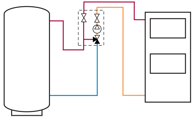
LK 864 - PUMP GROUP WITH THERMIC LOADING VALVE LK 823 THERMOVAR®.
