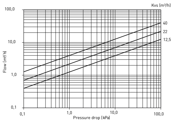
CAPACITY DIAGRAM
