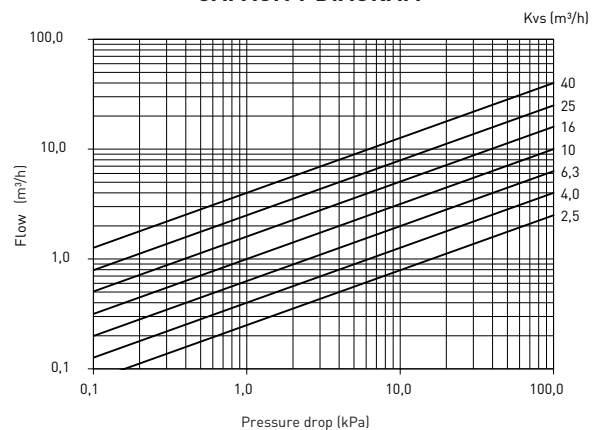
CAPACITY DIAGRAM
