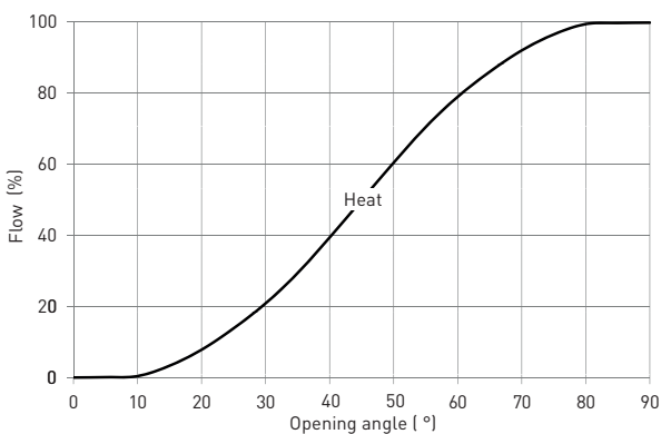
VALVE CHARACTERISTICS
