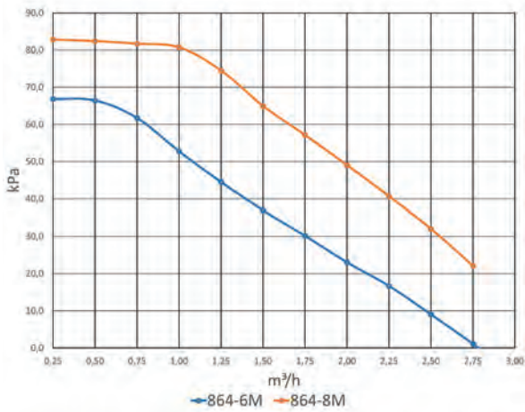
LK 864 - PUMP CHARACTERISTICS
