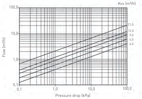
CAPACITY DIAGRAM
