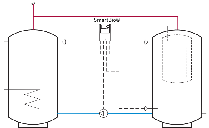
HYDRAULIC SYSTEM 3
