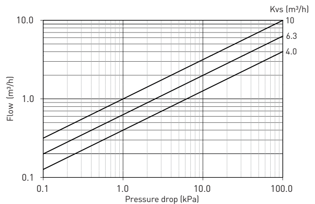
CAPACITY DIAGRAM
