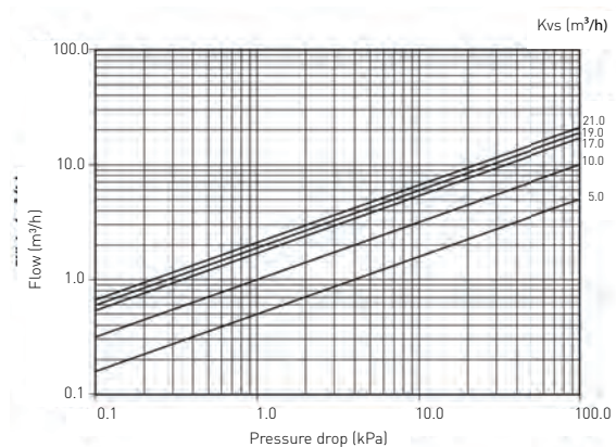
CAPACITY DIAGRAM - 0,5 MM
