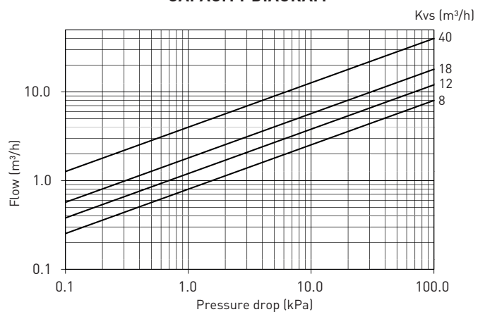
CAPACITY DIAGRAM
