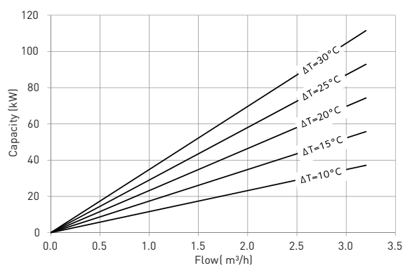
BOILER CAPACITY DIAGRAM, YONOS PARA*/7.5 RKC
