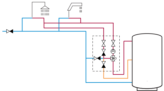
LK 865 - COMPLETE UNIT FOR HOT WATER CIRCULATION
